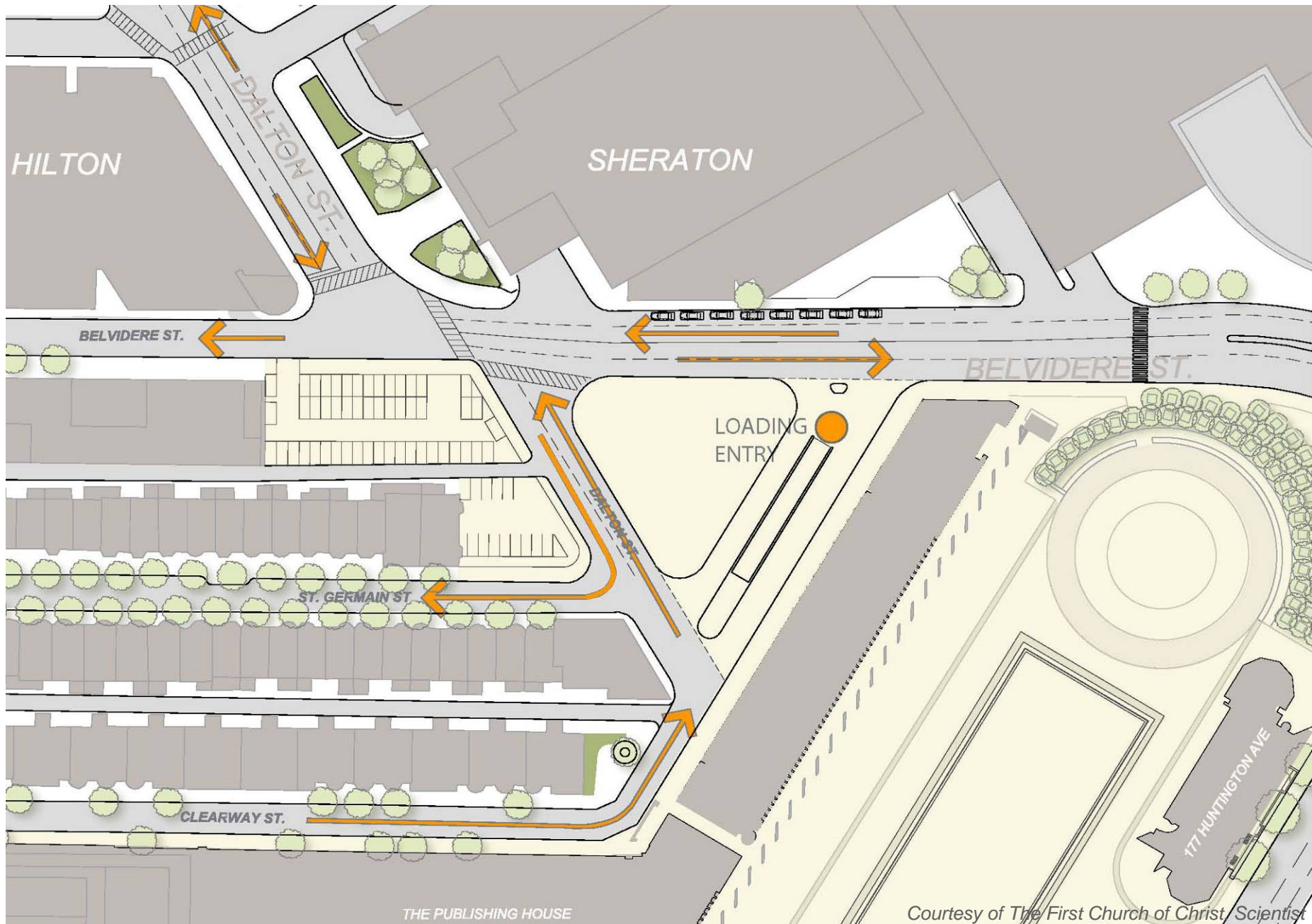
EXISTING BELVIDERE - DALTON SITE : Vehicular Circulation
