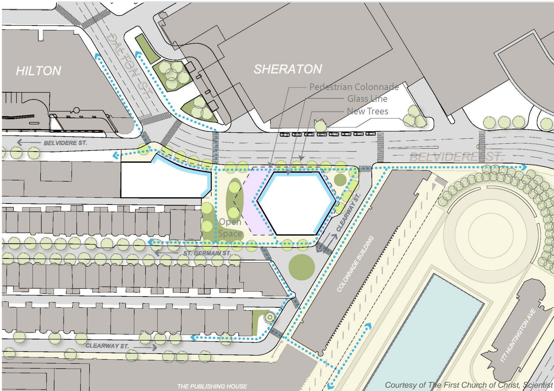
PROPOSED BELVIDERE - DALTON SITE : Pedestrian Flow & Circulation
