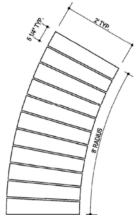
4 LONG CURVED BENCH WOOD SEAT PLAN 1" = 1'-0"
