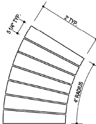
3 SHORT CURVED BENCH WOOD SEAT PLAN 1" = 1'-0"
