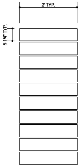
2 LONG STRAIGHT BENCH WOOD SEAT PLAN 1" = 1'-0"
