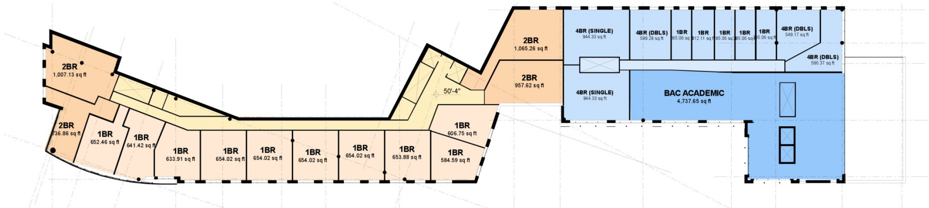
Third Floor
