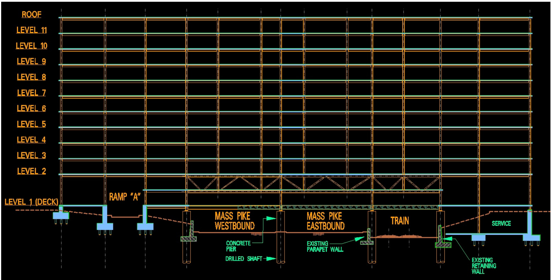
Structural Section
