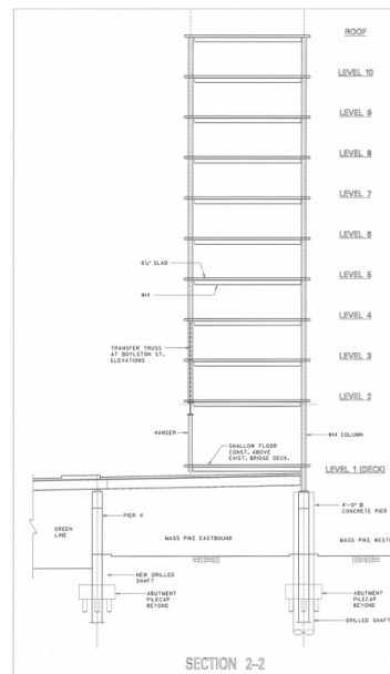
Structural Sections
