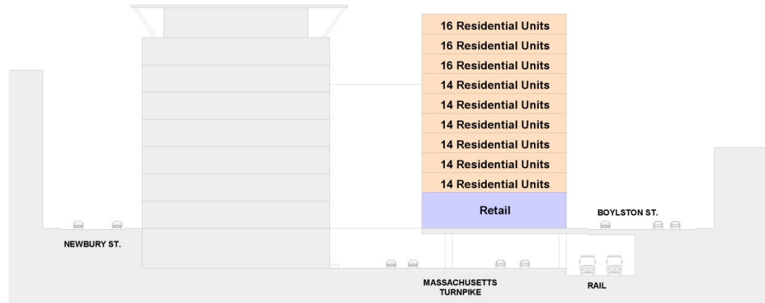
Building Sections
