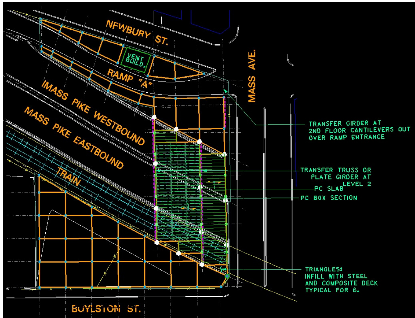
Composite Drawing of New Parcel 12 Deck and Foundations
