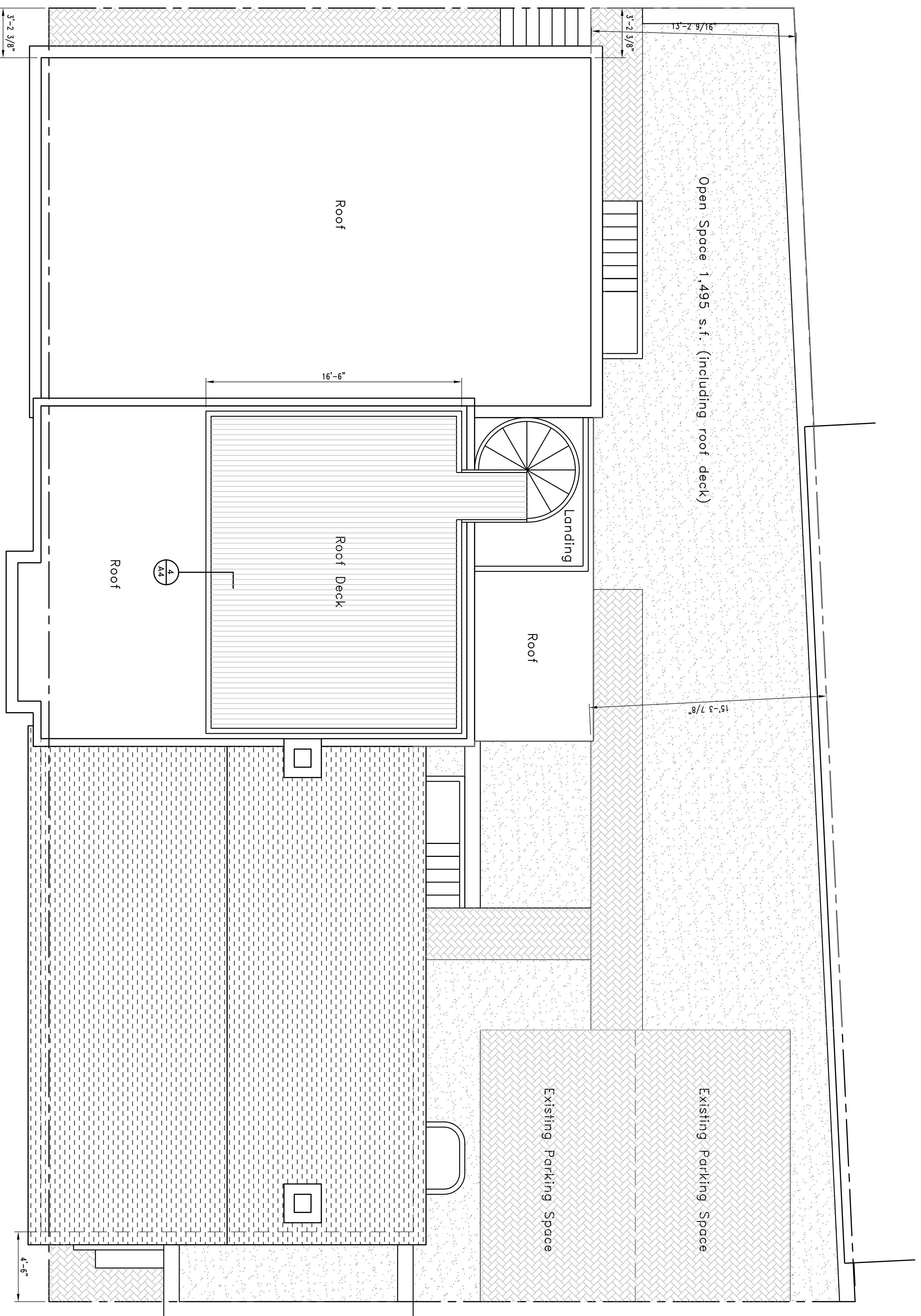
1 Architectural Site Plan Scale: 1/4" = 1'-0"
