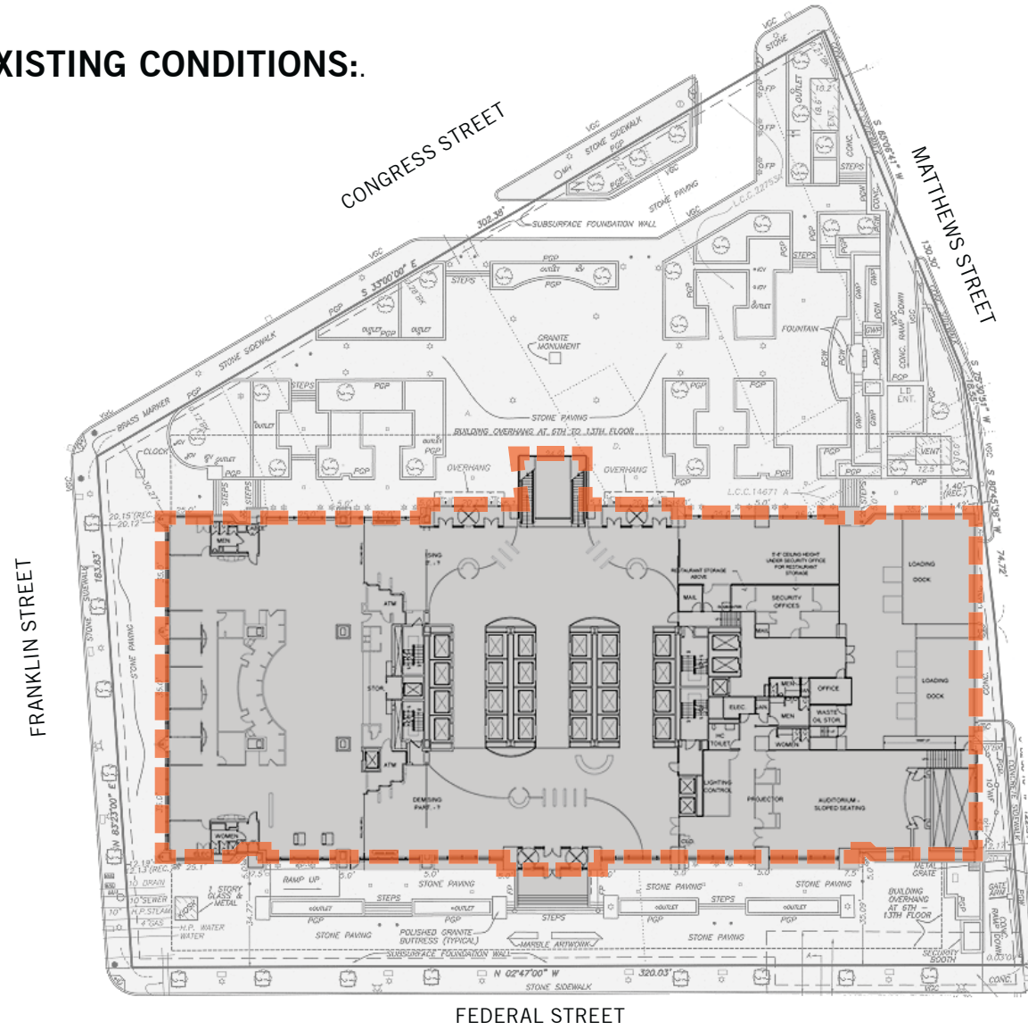
EXISTING STREET LEVEL FLOOR PLAN; N.T.S.
