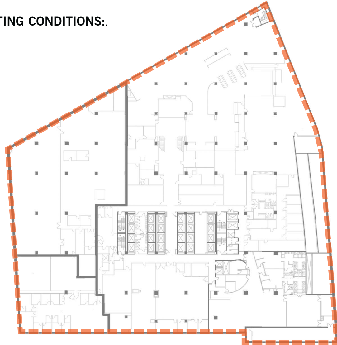
EXISTING 1st BASEMENT (B1) LEVEL FLOOR PLAN; N.T.S.
