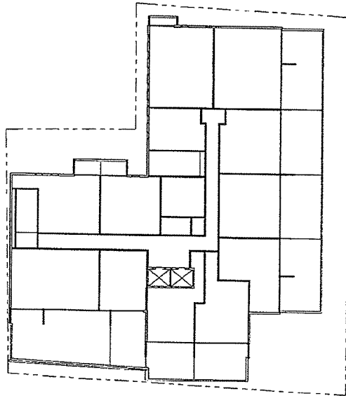
① Level 6 (Residential) 1/16" = 1'-0"
