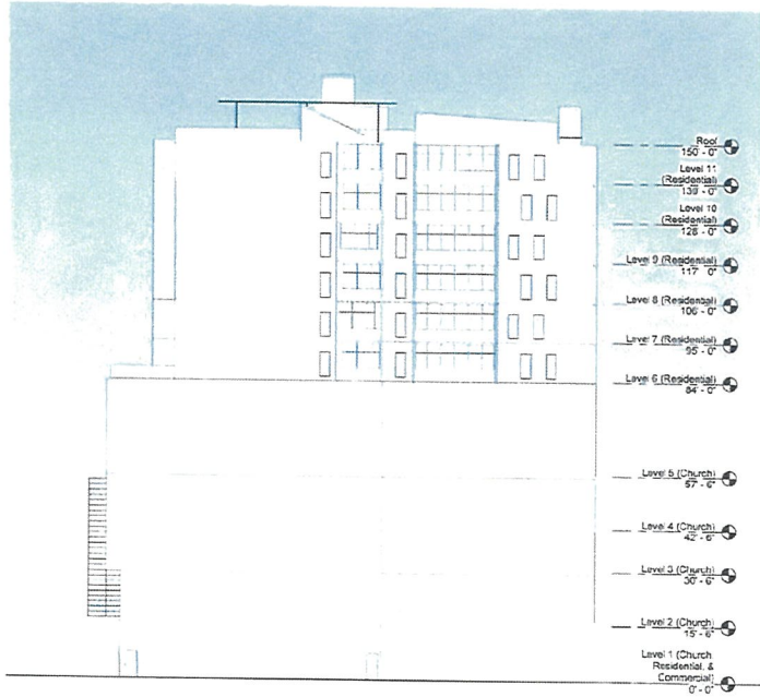
① East toward Washington St 1/16" = 1'-0"
