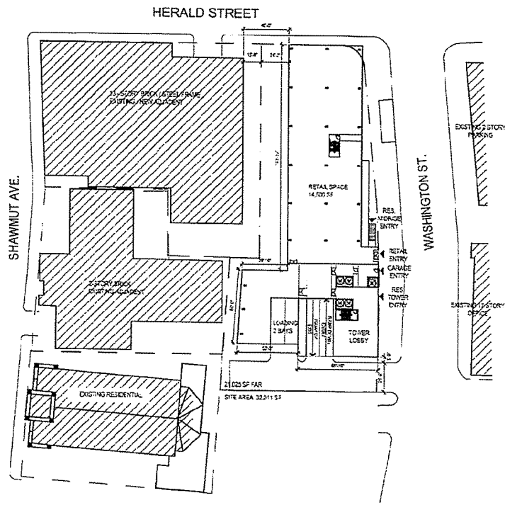
12 1st Level - Ground Floor Retail SCALE: 1/32" = 1'-0"
