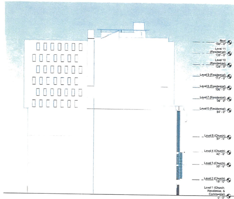
② North toward Herald St 1/16" = 1'-0"
