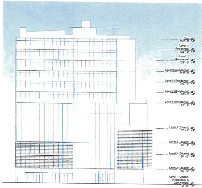
① West - Shawmut Ave 1/16" = 1'-0"
