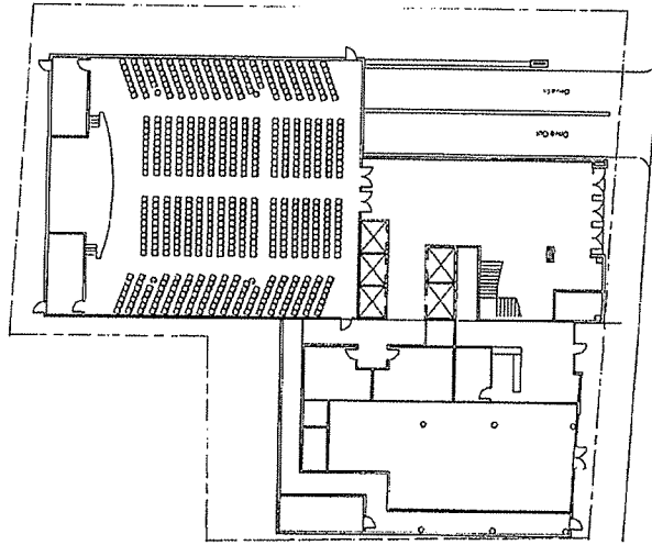
② Level 1 (Church, Residential, & Commercial) 1/16" = 1'-0"
