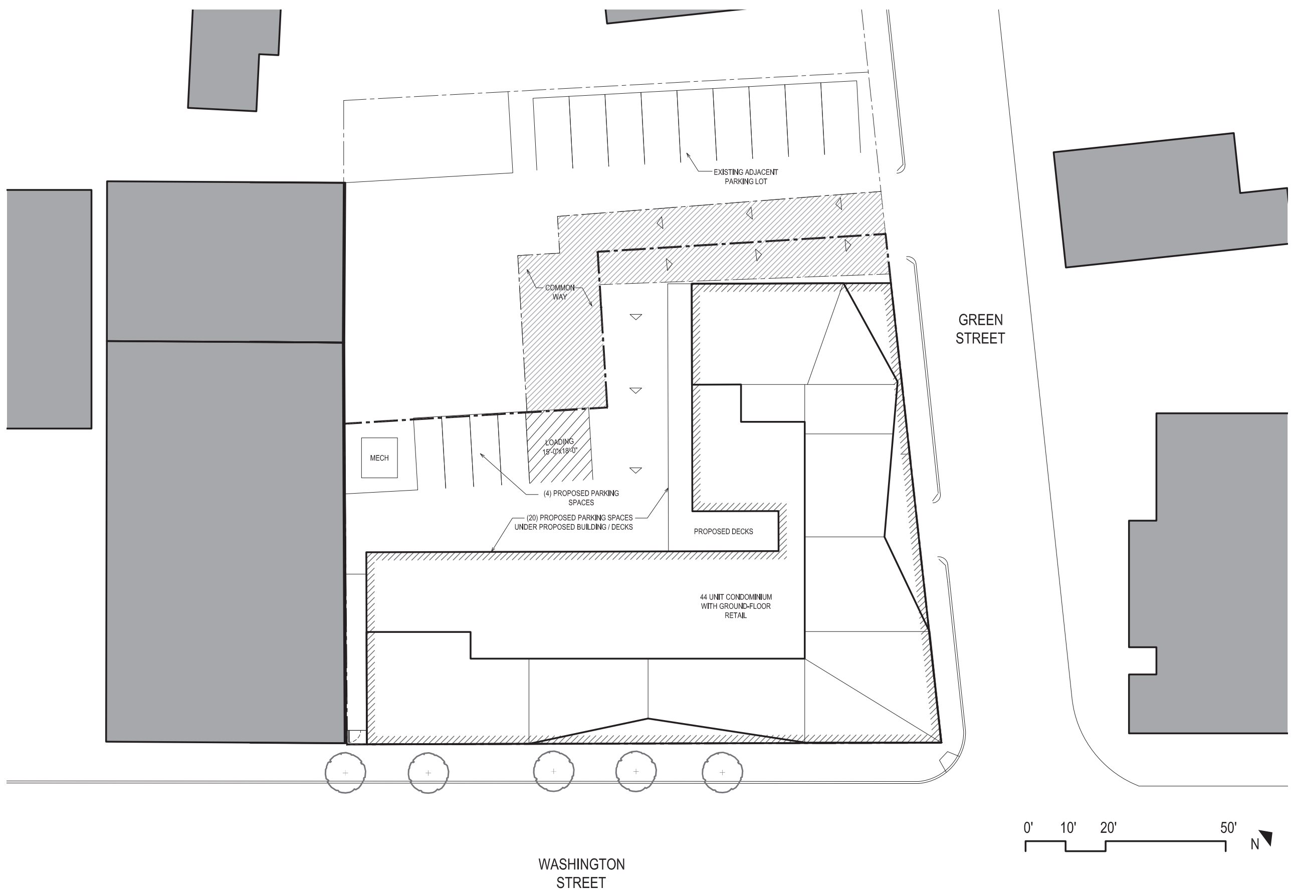
FIGURE 02 PROJECT SITE PLAN
